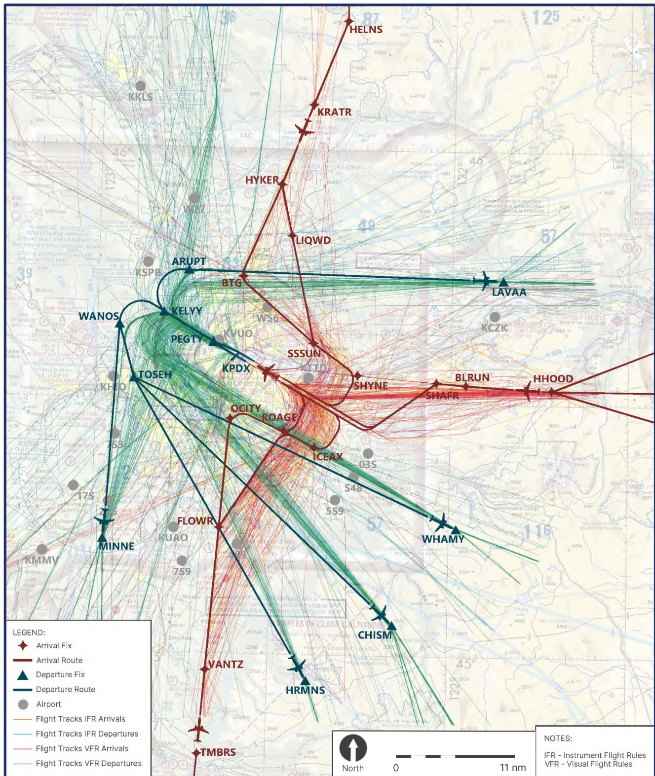
Exhibit 3-6 Published Arrival and Departure Routes – West Flow
